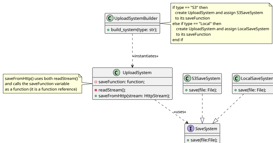
Figure 309: Possible class structure for a DI file upload
